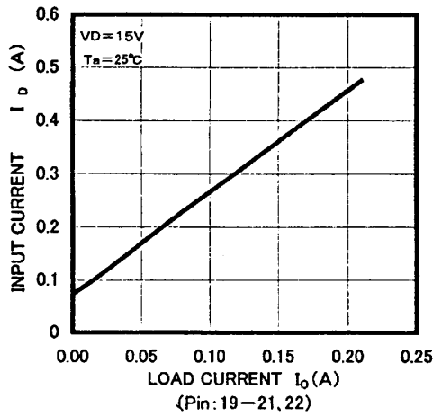
I_D - I_O CHARACTERISTICS (TYPICAL)
