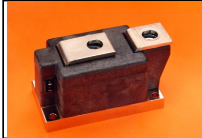
LS83_24 Single SCR POW-R-BLOK™ Module 240 Amperes / Up to 4000 Volts
