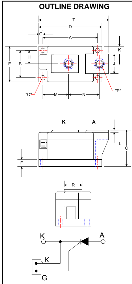
LS83_24 Single SCR POW-R-BLOK™ Module 240 Amperes / Up to 4000 Volts
